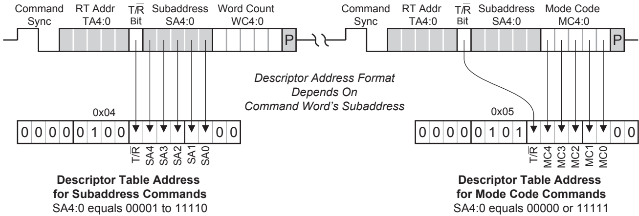
Figure 11. Deriving a Descriptor Table Control Word Address From Command Word (assumes table base address = 0x0400)
