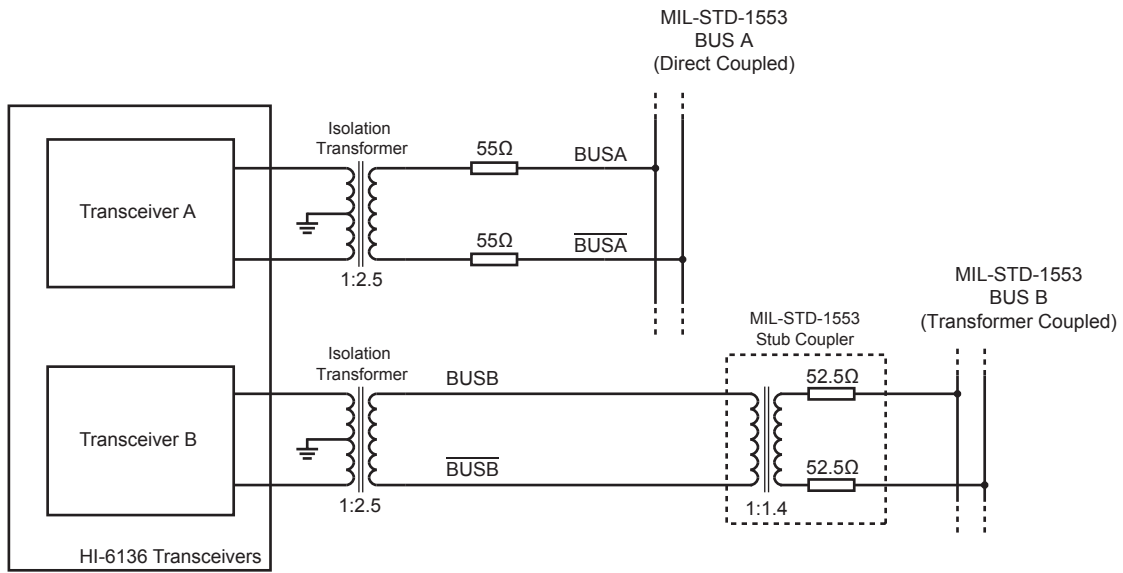
Figure 25. Bus Connection Example using HI-6136
