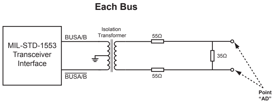
Figure 26. MIL-STD-1553 Direct Coupled Test Circuits
