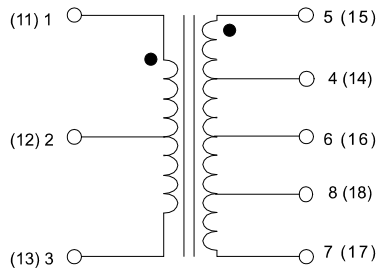
SCHEMATIC "11"
