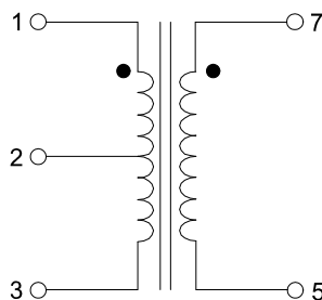
SCHEMATIC "18"
