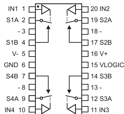
HI-8200PSHF 20-Pin TSSOP package
